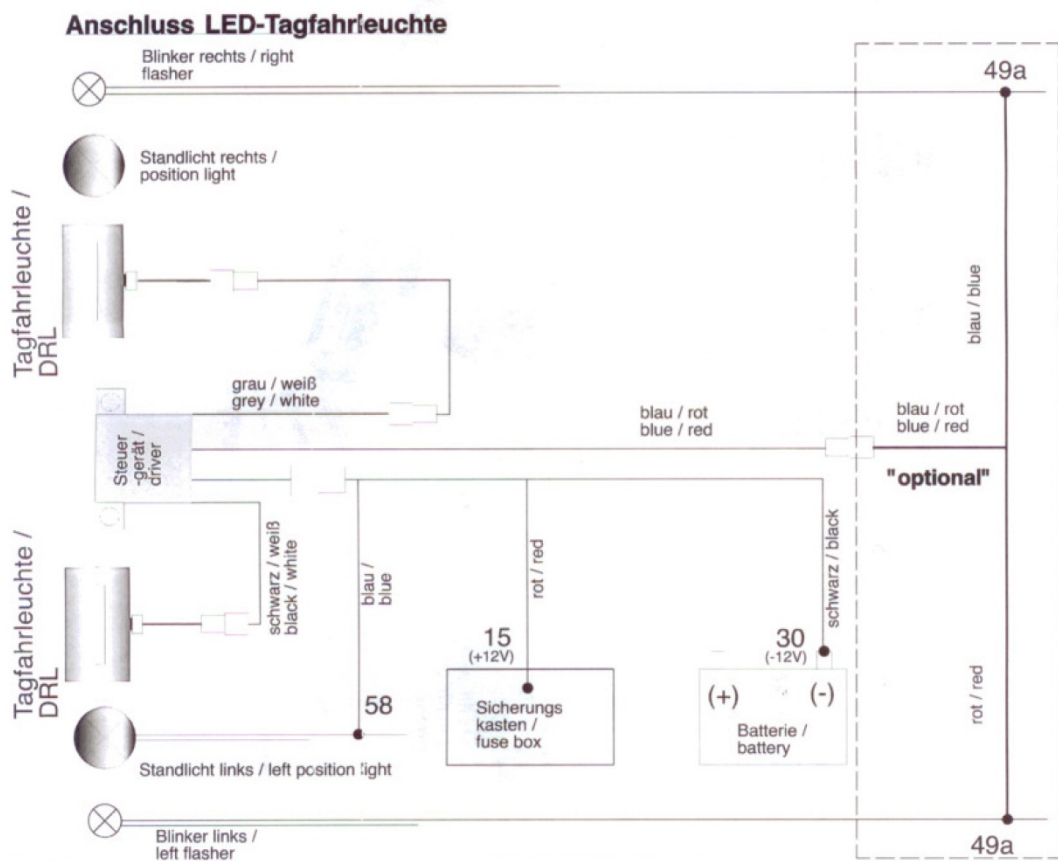
Bild 6: Anschlußplan Figure 6: Connecting plan
